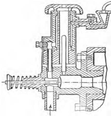
FIG. 321.—The Blackstone Kerosene Vaporizer. As is evident, the oil sprayed in at the right-hand top of the cylinder passes through an annular space around the "chimney" of the hot tube, passing thence to the space behind the inlet valve.
